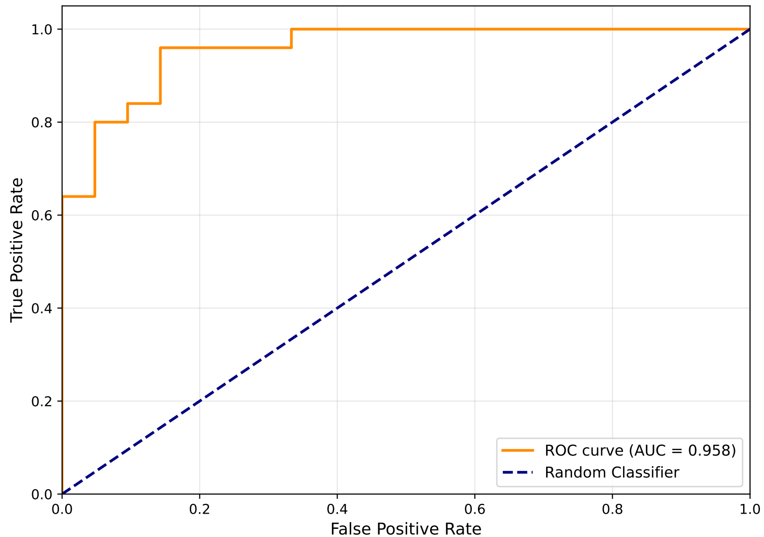
ROC Curve for Tuned Extra Trees
